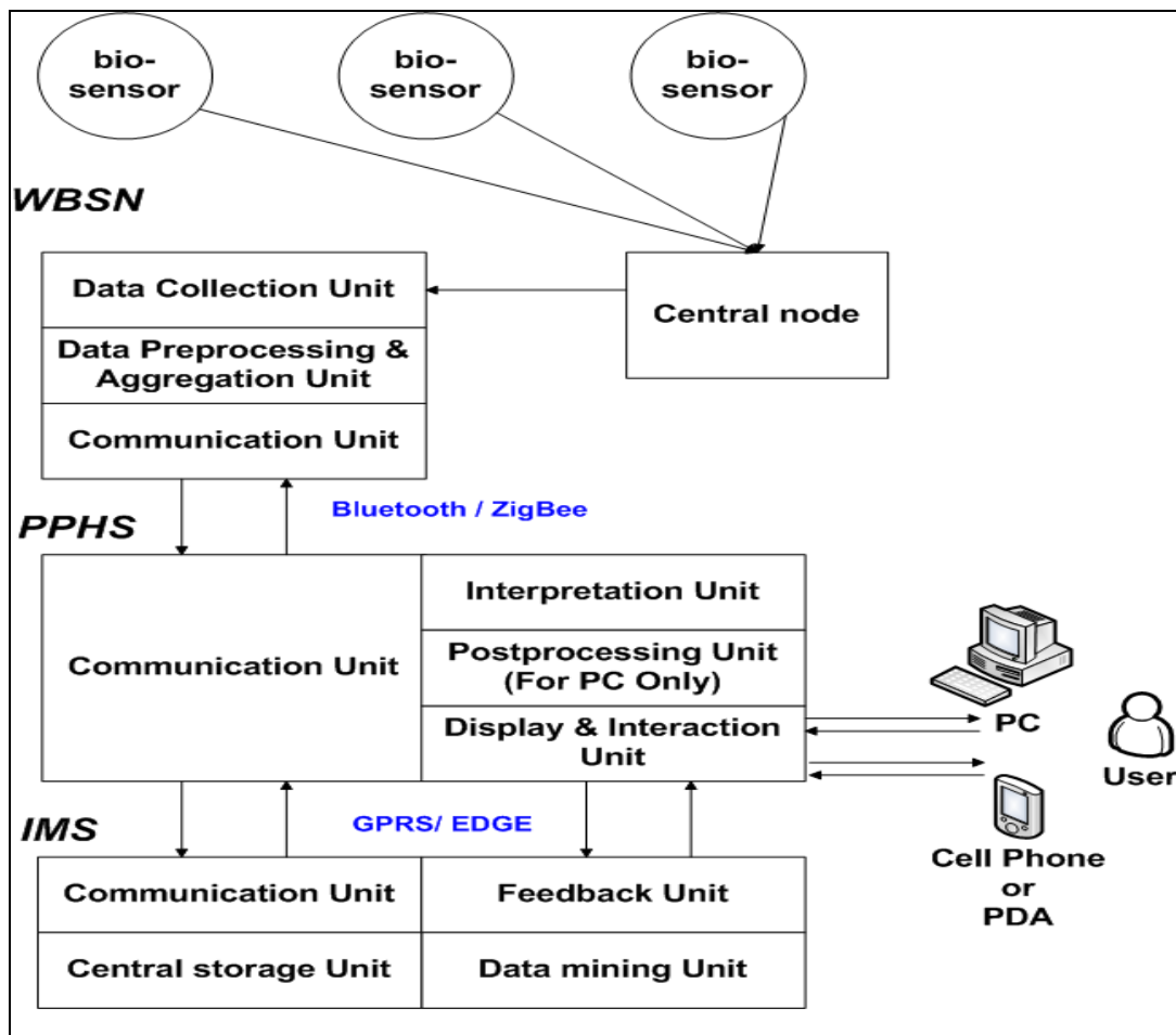
Figure 2. IMHMS System Architecture
